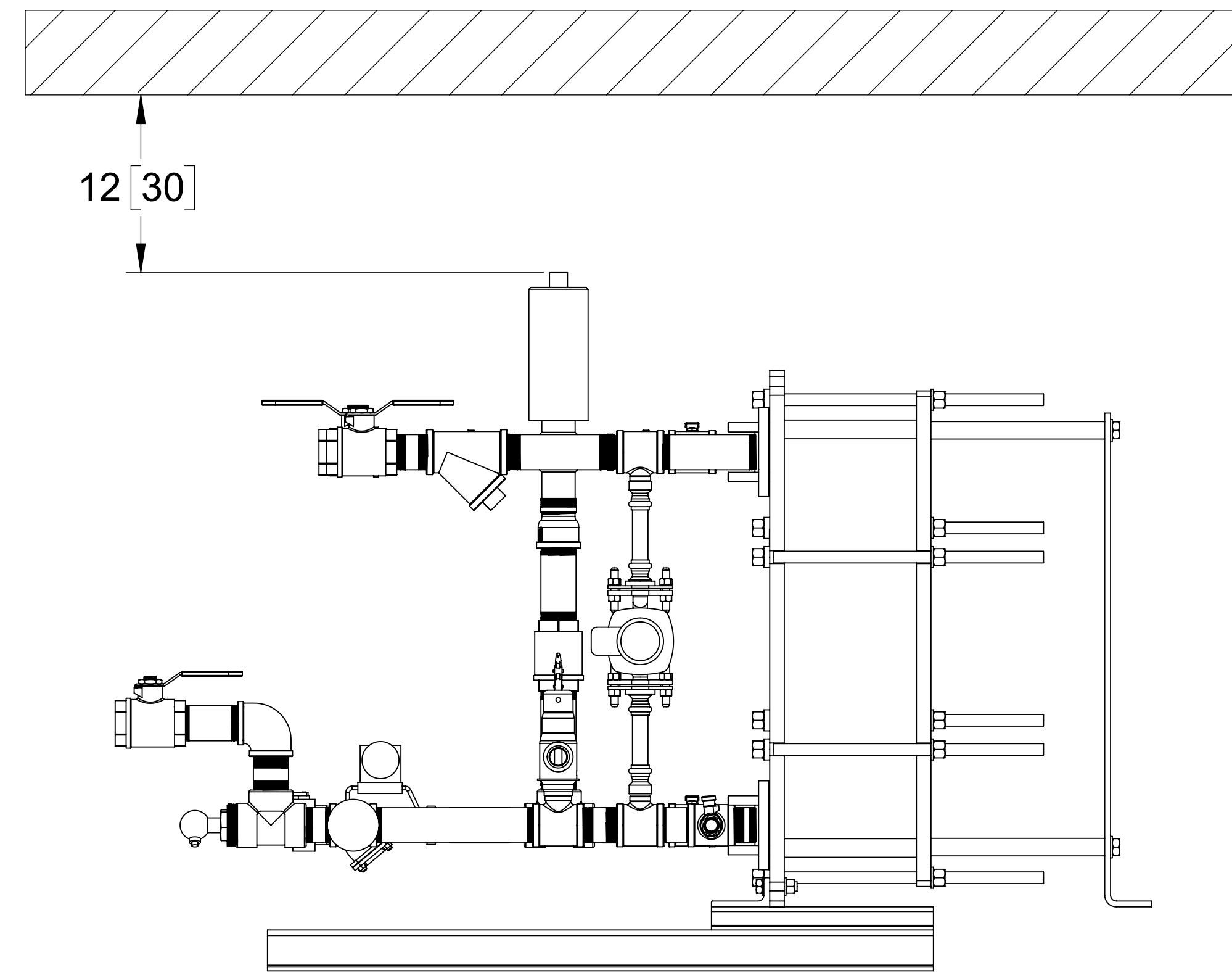
ELEVATION VIEW
