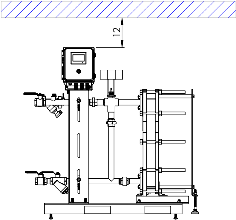
ELEVATION VIEW
